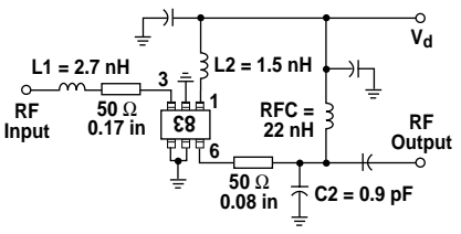
Figure 27. Schematic Diagram of 2.5 GHz Amplifier.
